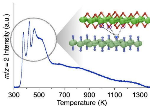
Figure 1. A representative multimodal H 2 -TPD profile of HB nanosheets with a schematic illustration of interlayer H \cdots H distances.
