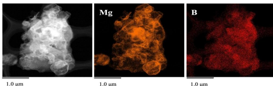
Figure 1. STEM and EDS mapping of highly dispersed Mg on boron nanosheets.
