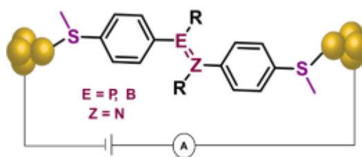
Figure 1. Boron and pnictogen molecular electronics
